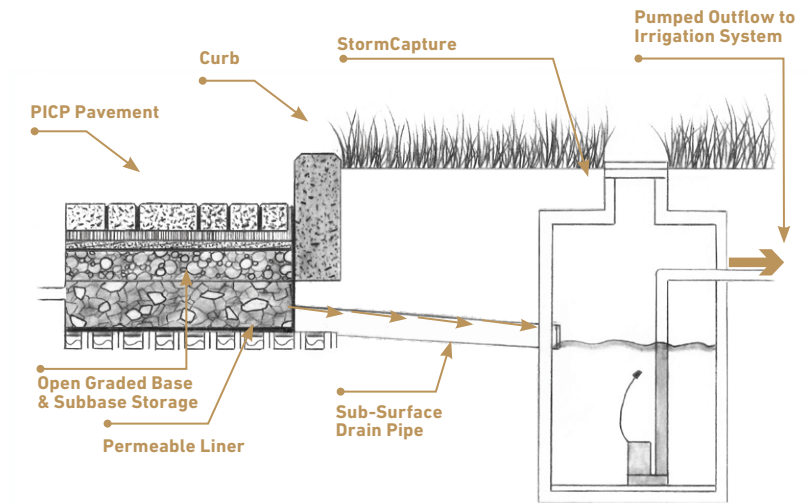
Water Harvesting Using PICP
